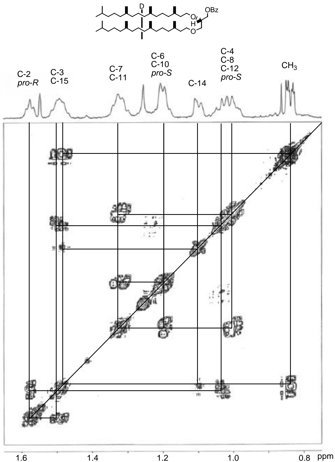
^1\text{H} - ^1\text{H} COSY spectrum (500 MHz, \text{CDCl}_3 ) of multiply deuterated diphytanylglycerol benzoate from M. jannaschii
