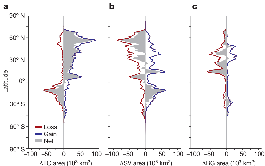
Figure 4.5 | Diagrams showing latitudinal profiles of land cover change over the period 1982 to 2016 based on analysis of time-series of NOAA AVHRR imagery: a) tree canopy cover change ( \Delta\text{TC} ); b) short vegetation cover change ( \Delta\text{SV} ); c) bare ground cover change ( \Delta\text{BG} ). Area statistics were calculated for every 1^\circ of latitude (Song et al. 2018). Source of data: NOAA AVHRR.
