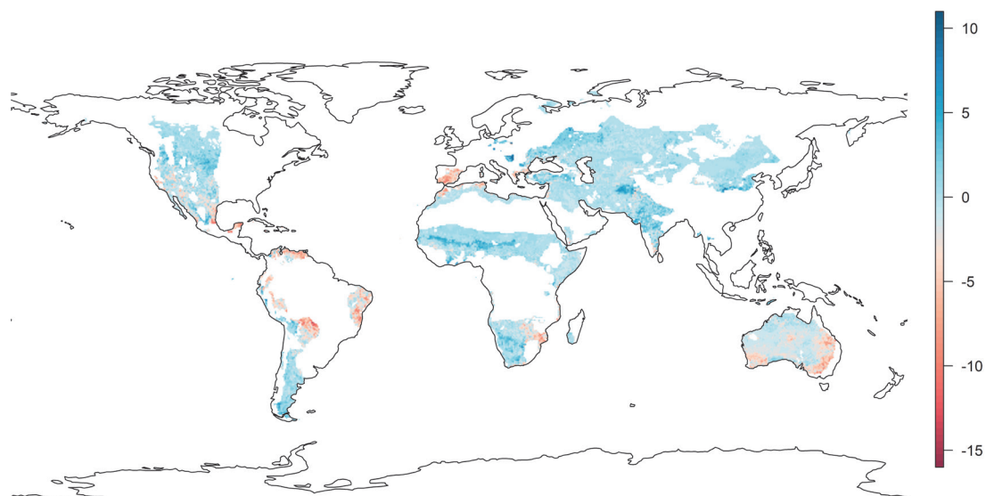
Figure 3.14 | Difference between the number of invasive alien species (n=99, from Bellard et al. (2013)) predicted to occur by 2050 (under A1B scenario) and current period '2000' within the dryland areas.
