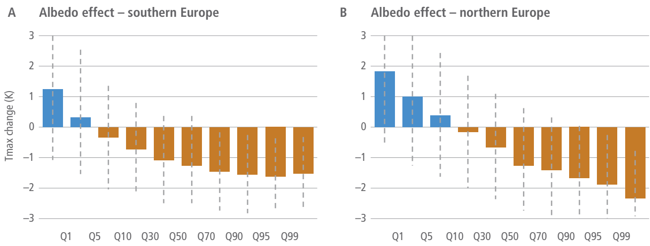
Figure 2.19 | Change in summer (July–August) daily maximum temperature (°C) resulting from increased surface albedo in unploughed versus ploughed land, in (A) southern, and (B) northern Europe, during the period 1986–2009. Changes are simulated for different quantiles of the daily maximum temperature distribution, where Q1 represents the coolest 1% and Q99 the warmest 1% of summer days. Only grid cells with more than 60% of their area in cropland are included. The dashed bars represent the standard deviation calculated across all days and grid points. Southern Europe refers to Europe below 45°N, and northern Europe refers to Europe above 45°N (Davin et al., 2014).
