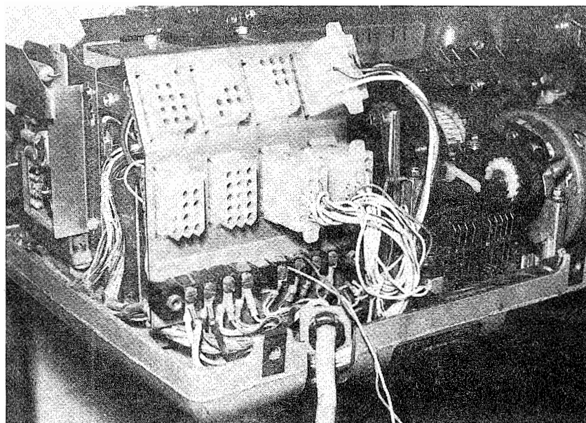
VIEW OF MODEL 33 WITH COVER REMOVED
