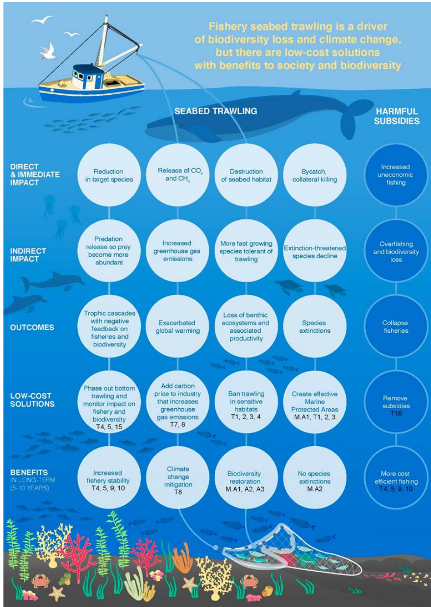
Figure A1.4 Illustration of the multiple direct and indirect negative impacts of seabed trawling on target and extinction-endangered species, habitats and greenhouse gases emissions. The removal of harmful fisheries subsidies and low-cost management actions, including protected areas, can help restore biodiversity, benefit food and socio-economic security and mitigate against future climate change. Abbreviations M and T refer to the Milestones and Targets of the draft post-2020 global biodiversity framework.
