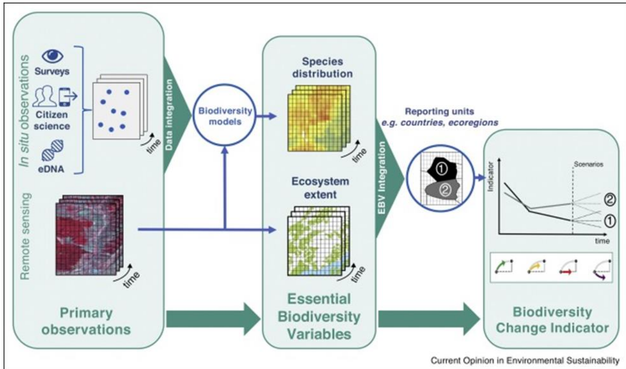
Figure 4.2 General workflow from multiple primary biodiversity observations, to standardised essential biodiversity variables and to biodiversity change indicators (Source: Navarro et al. 2017). Expert knowledge and assessment are essential for the harmonisation of data across sources and spatial scales.
