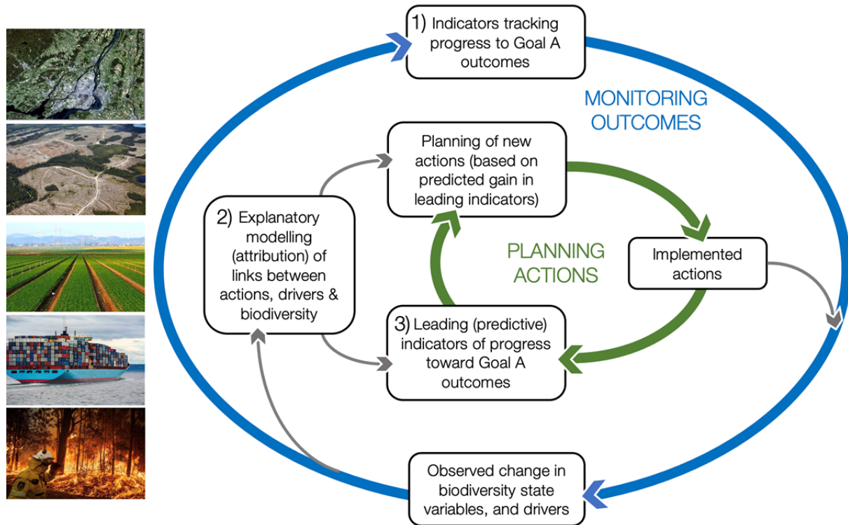
Figure 6. The iterative cycle of monitoring and action guided by explanatory models and indicators. The outer blue cycle refers to the monitoring of actual changes in biodiversity and the updates in indicators used to track progress to Goal A outcomes (box 1). The inner cycle refers to the role of explanatory models (box 2) that use component and complementary indicators that include indicators for drivers and actions and leading indicators (box 3) that incorporate an understanding of the impacts of drivers (attribution) on trends in essential biodiversity variables to guide spatial planning and the prioritization of conservation action.
