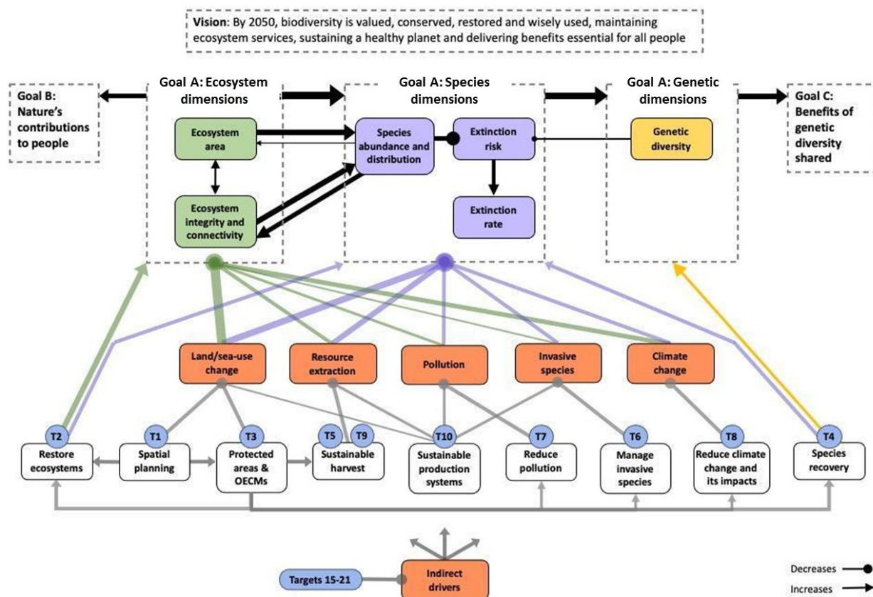
Figure A1.2 Extended version of Figure 1.1 in section 1.3.1. This figure shows the relationship between outcomes (Goals and Goal A components, in dashed boxes), dimensions of biodiversity (A1 area, integrity and connectivity of natural ecosystems, green; A2 abundance and distribution of populations of species, species extinction rate and species extinction risk, purple; and A3 maintenance of genetic diversity, gold boxes), direct drivers (orange boxes) and targets (blue circles, where T1 is Target 1, and so forth). Relationships amongst goals and Goal A components and dimensions of biodiversity are shown by black arrows, labeled with letters:
