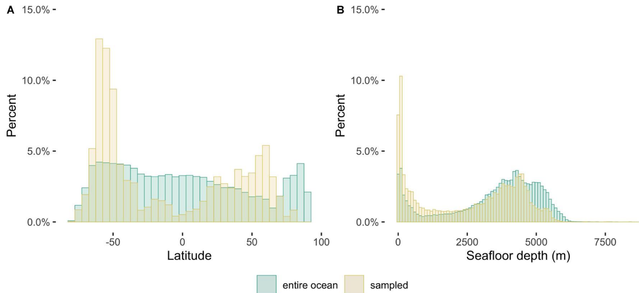
Figure 4.6 Overlap between sampled sites and the global ocean. Histograms of latitude (A) and seafloor depth (B) for the global ocean area (“entire ocean”) compared with areas sampled by observing programs in this study (“sampled”). Results include the spatial information from the surveyed programs and the datasets from the Ocean Biodiversity Information System (OBIS) and the Global Biodiversity Information System (GBIF). Bin widths are 5 degrees for latitude (A) and 100 meters for seafloor depth (B). Regions that were under sampled are characterised by the entire ocean (blue bars) being greater than the sampled areas (gold bars), with the converse for oversampled areas (Source: Satterthwaite et al. 2021).
