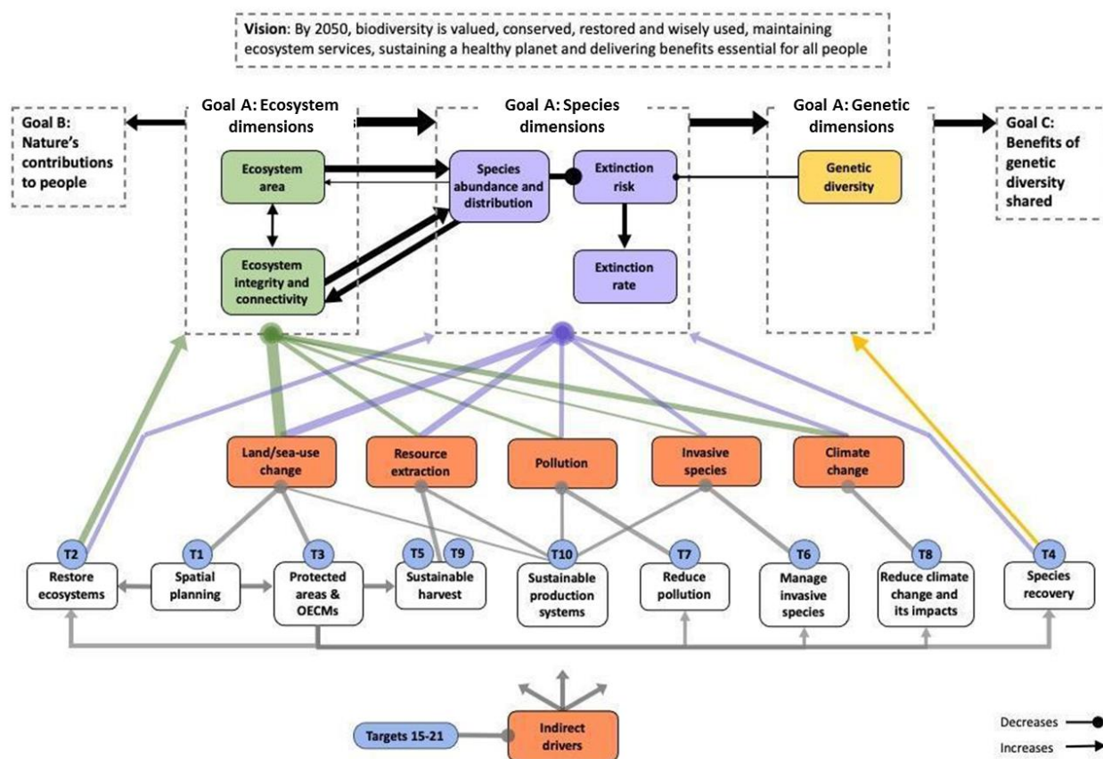
Figure 1.1 Relationship between outcomes, components of biodiversity, direct drivers and targets of the GBF. This figure shows the relationship between outcomes (Goals and Goal A components, in dashed boxes), components of biodiversity (A1 area, integrity and connectivity of natural ecosystems, green; A2 abundance and distribution of populations of species, species extinction rate and species extinction risk, purple; and A3 maintenance of genetic diversity, gold boxes), direct drivers (orange boxes) and targets (blue circles, where T1 is Target 1, and so forth). See Table 1.1 for wording of goal A, milestones and targets. Black arrows depict relationships amongst goals and goal A components highlighting the role of biodiversity (Goal A) in sustaining ecological functions, ecosystem services and Nature’s contributions for people (Goal B) and the genetic diversity that underpins Goal C. Relationships between dimensions of biodiversity, direct drivers and targets are shown in coloured and grey arrows where arrow weight is relative to impact in Figure 1.3 (also in Figure 2, see Appendices 1.1 and 1.2 for documentation). Some targets act
