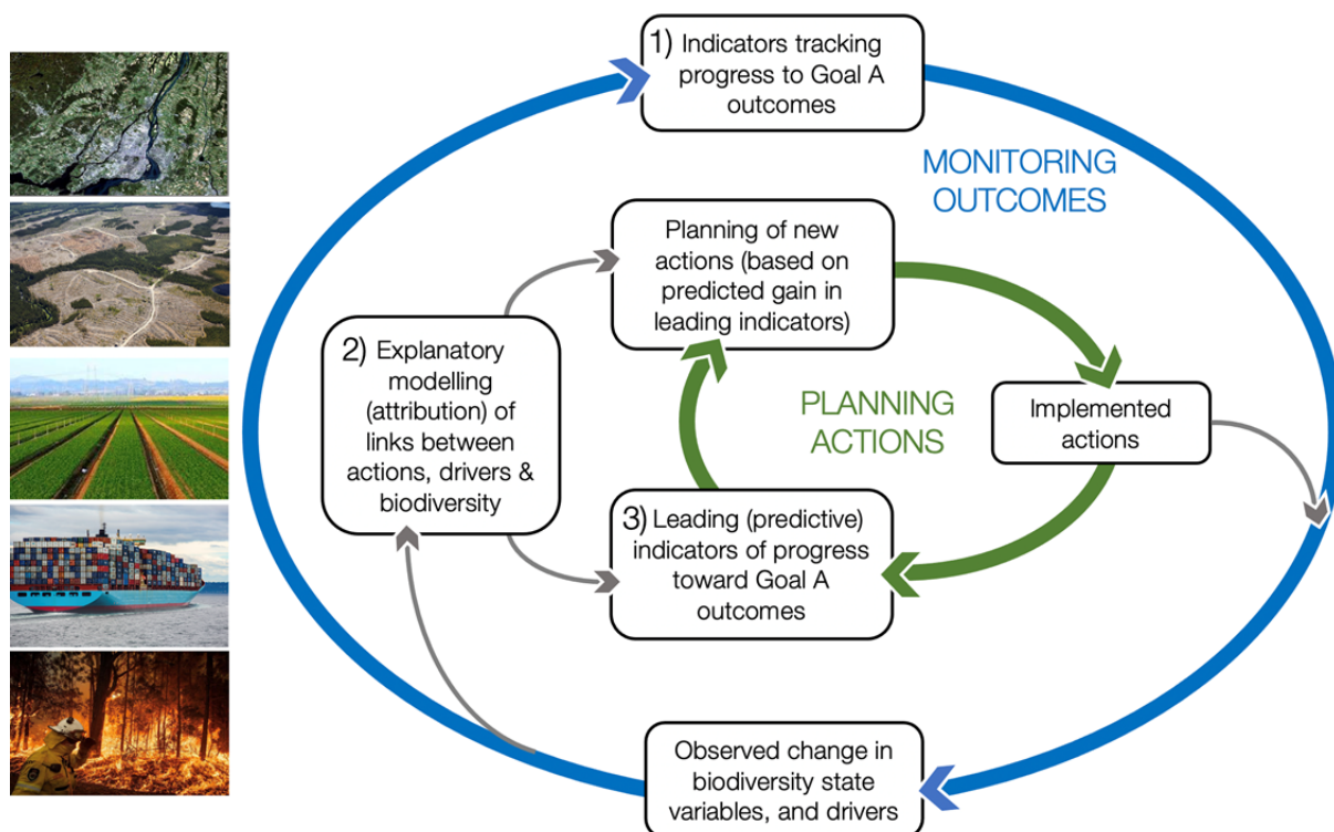
Figure 4.1 The iterative cycle of monitoring and action guided by explanatory models and indicators. The outer blue cycle refers to monitoring of actual changes in biodiversity and the updates in indicators used to track progress to Goal A outcomes (box 1). The inner cycle refers to the role of explanatory models (box 2) and leading indicators (box 3) that incorporate understanding of the impacts of drivers (attribution) on trends in essential biodiversity variables to guide spatial planning and prioritization of conservation action.
