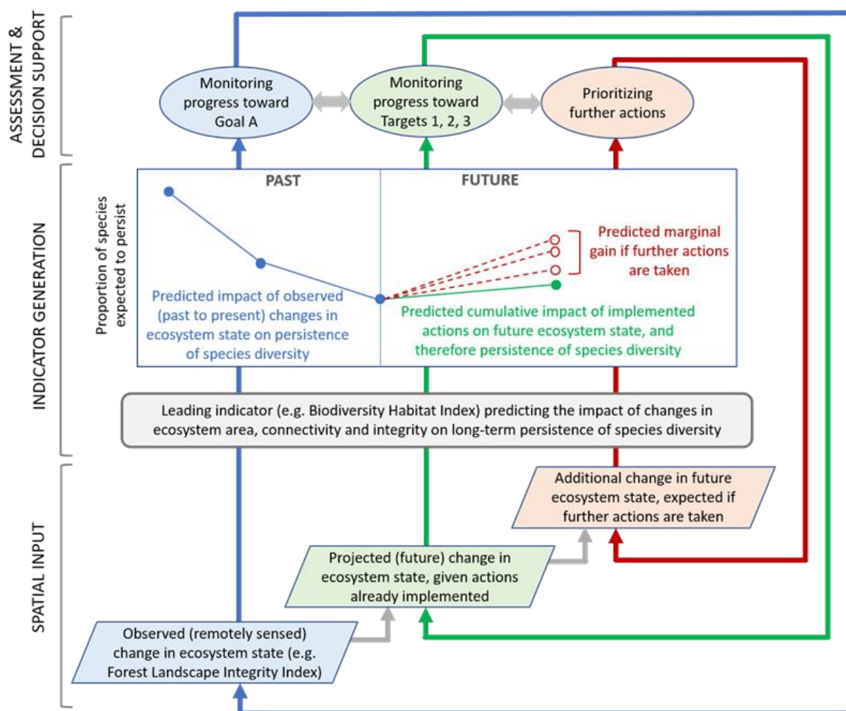
Figure 4.9 An example of how a leading indicator, in this case the Biodiversity Habitat index (Hoskins et al. 2020; Hansen et al. 2021), could be used to integrate monitoring of progress toward Goal A with monitoring and prioritization of area-based actions under Targets 1, 2 and 3.
