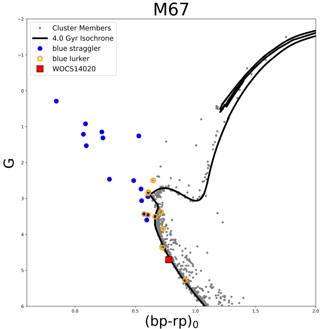
Figure 1. Color-magnitude diagram of M67 highlighting Gaia DR3 proper-motion members (gray), blue stragglers (blue), BLs (orange), and our target, the BL WOCS 14020 (red square). Memberships are determined as described in Leiner & Geller (2021)
