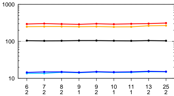
BLOSUM80
