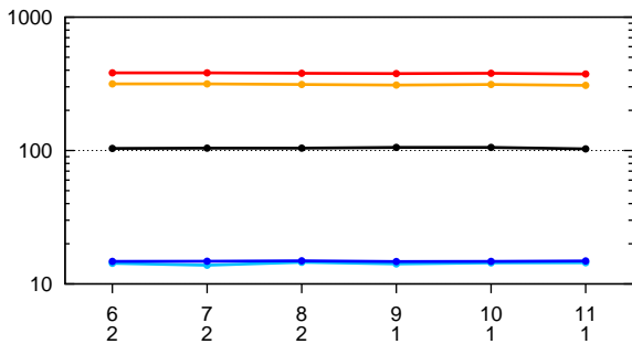
PAM70
