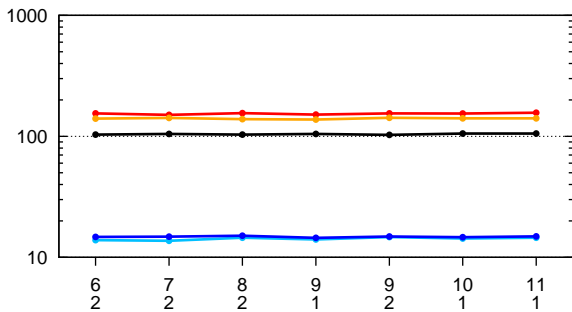
BLOSUM90
