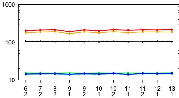
BLOSUM62
