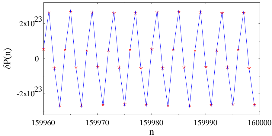
Fig. 11. Result of (12), shown by the blue line, using only the pair of orbits of generation 2 (with f_2 = 4 ), in the region near n = 160,000 . The exact \delta P(n) = P(n) - P_{as}(n) are shown by the red stars. Note that the beat structure in the exact \delta P(n) has practically disappeared.
