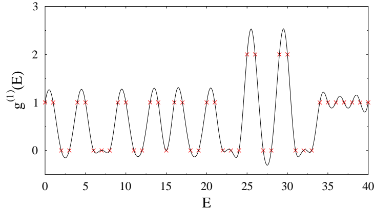
Fig. 2. Bessel-smoothed partition density g^{(1)}(E) (7) (black line) for small energies E . The red crosses at integer values E = n show the exact values of P(n) .
