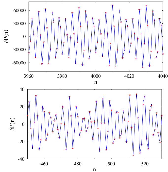
Fig. 8. Same as Fig. 7 in two regions of small n .
