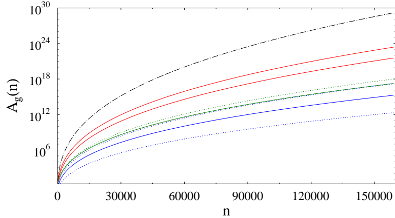
Fig. 9. Semiclassical amplitudes A_g(n) for the generations (from top to bottom) 0 (giving the smooth part), 2, 1, 6+7, 3+4+5, 8, 10, 9 (see text for details).
