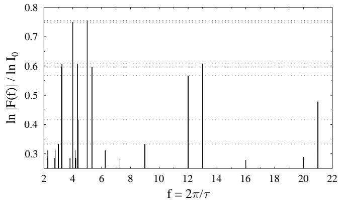
Fig. 4. Scaled Fourier transform \ln |F(f)| of g(E) on a logarithmic vertical scale. The horizontal dashed lines give the calculated relative intensities of the first 10 generations.
