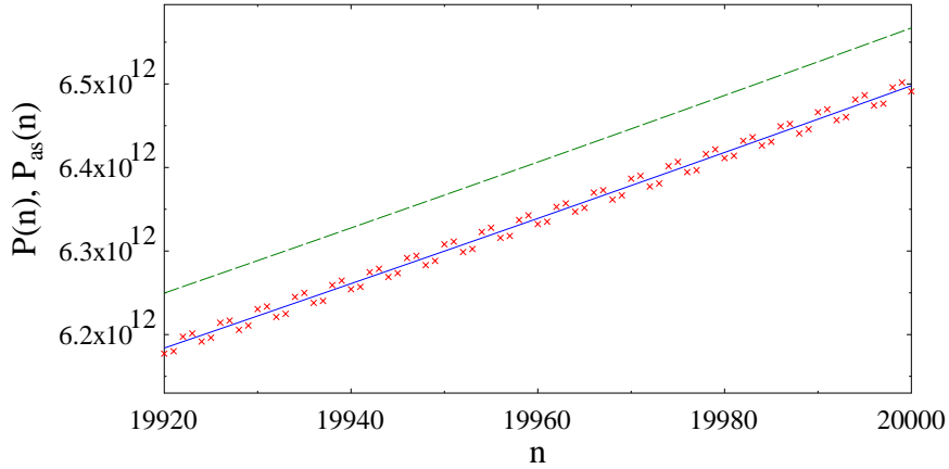
Fig. 3. Exact P(n) by crosses (red), leading-order asymptotic part P_{as}^{(0)}(n) (8) by the dashed (green) line, and corrected asymptotic part P_{as}(n) (9) by the solid (blue) line in the large- n region.
