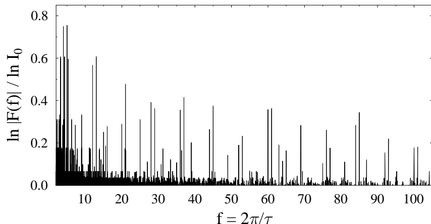
Fig. 5. Same as Fig. 4 over a larger range of the frequency f .
