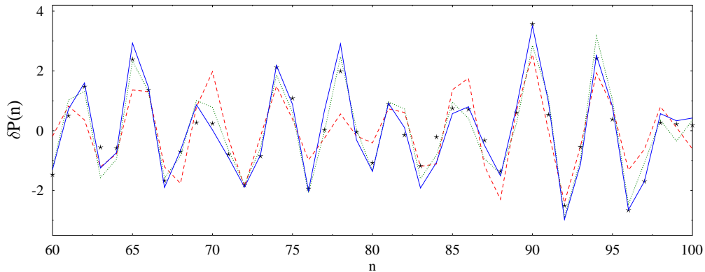
Fig. 10. Result of trace formula (12) around n = 80 for increasing numbers of generations included. Dashed line (red): generations 1 and 2; dotted line (green): generations 1-7; solid line (blue): generations 1-10. The stars (black) show the exact \delta P(n) .
