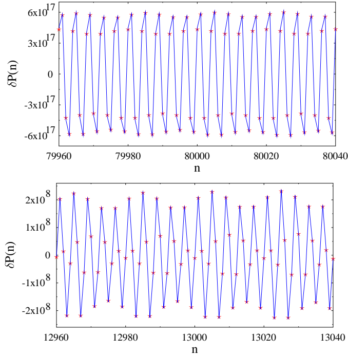
Fig. 7. Result of the trace formula (12), shown by blue lines, versus the exact \delta P(n) = P(n) - P_{as}(n) , shown by red stars, in two regions of large n .
