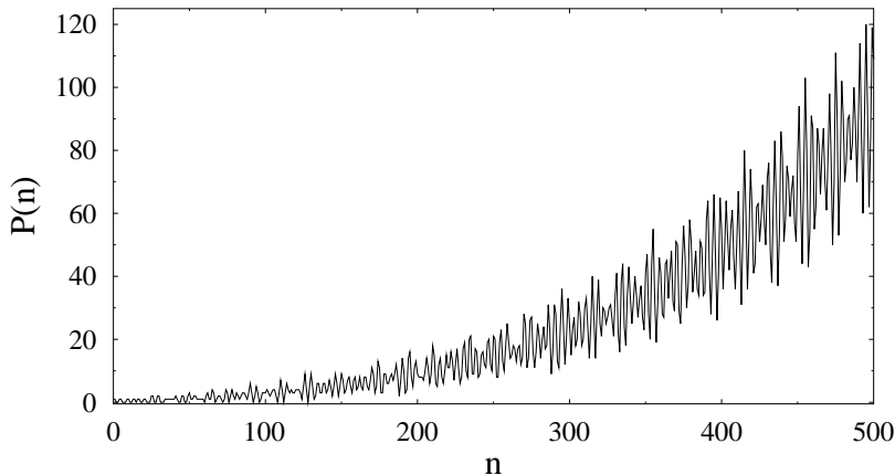
Fig. 1. P(n) of the distinct square partitions shown in the low- n region. Note that P(n) is defined for integer values of n . Here we have joined the points by a continuous curve to emphasize the beat structure.
