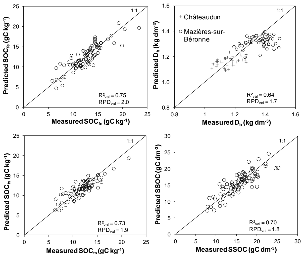
Figure 5. Comparison between conventionally determined and VNIRS predicted values of \text{SOC}_{\text{fe}} (fine earth), \text{SOC}_{\text{ts}} (total soil), D_b and SOC stock (SSOC) for validation samples (predictions made using the whole 350-2500 nm range; distinction between both sites was hardly possible except for D_b ).
