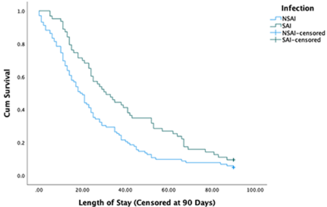
Survival Functions
