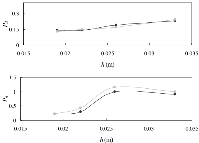
Figure 20 Phase difference ( P_d ) corresponding to velocity (first panel) and force (second panel). Lines as described in previous figure
