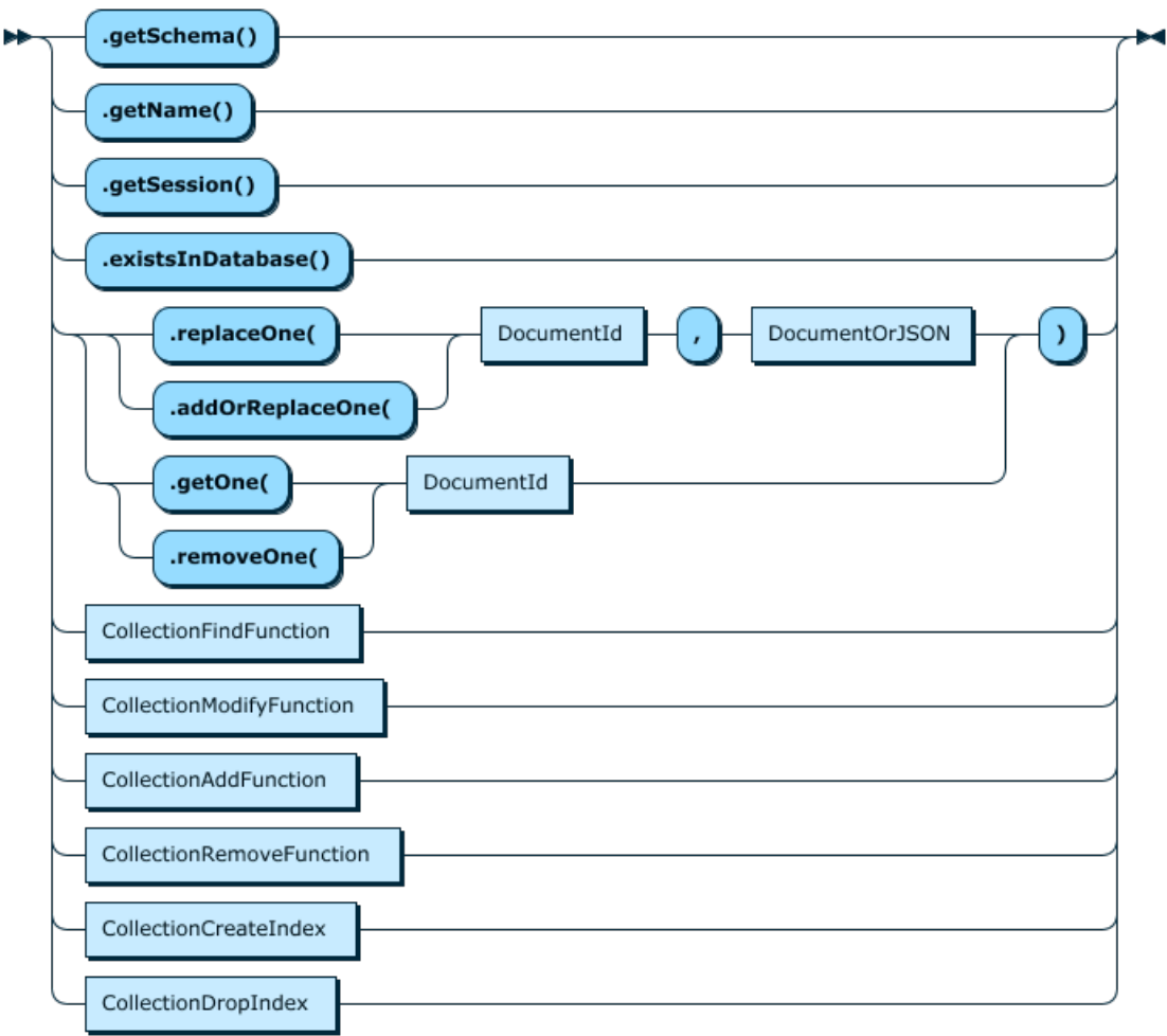
Figure 11.7 Collection
