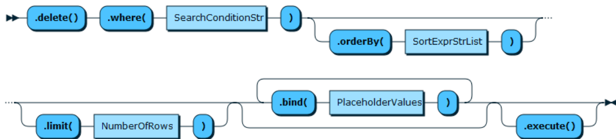
Figure 11.18 TableDeleteFunction
