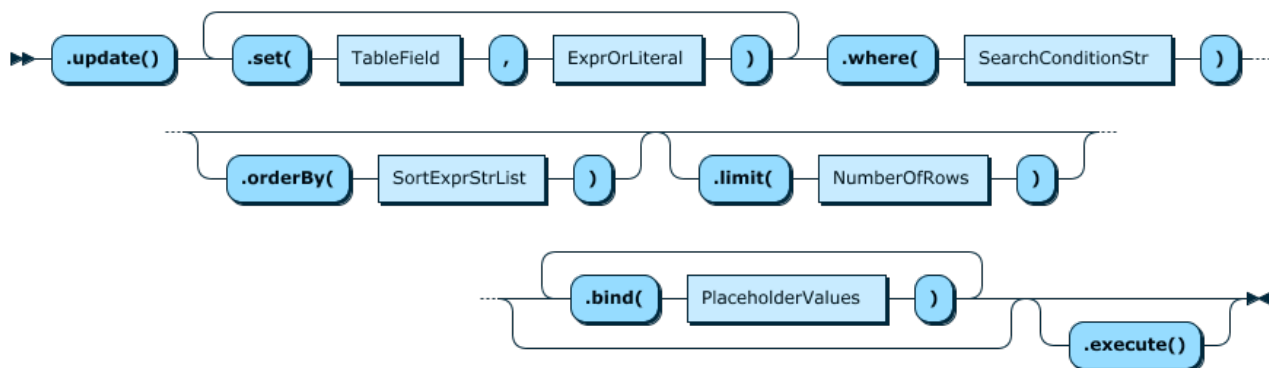
Figure 11.17 TableUpdateFunction
