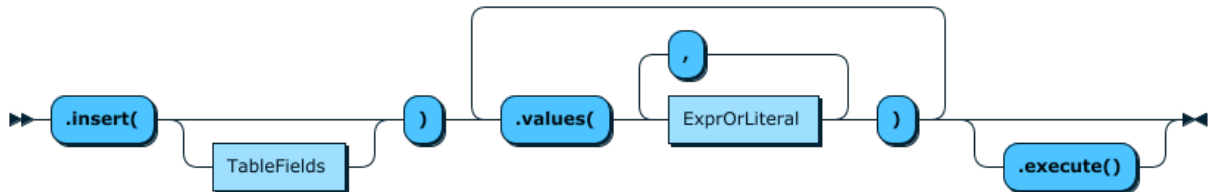
Figure 11.16 TableInsertFunction
