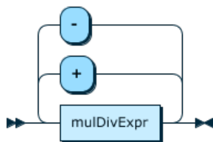
Figure 12.24 addSubExpr
