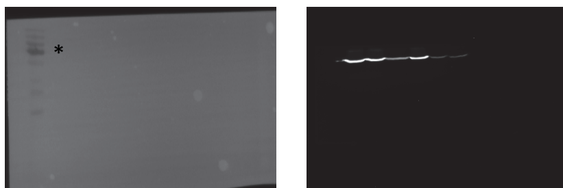
Fig. 2C Phospho- STAT3
