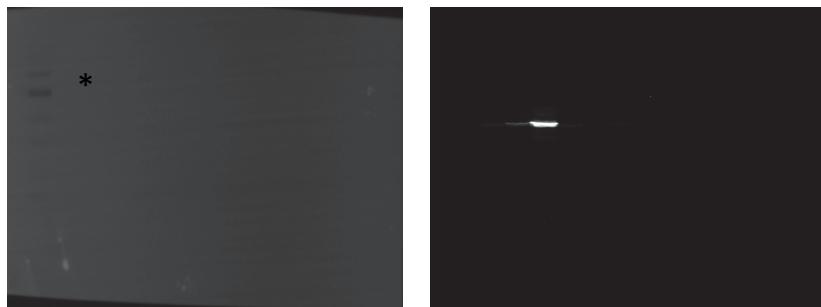
Fig. 2C Phospho- STAT1
