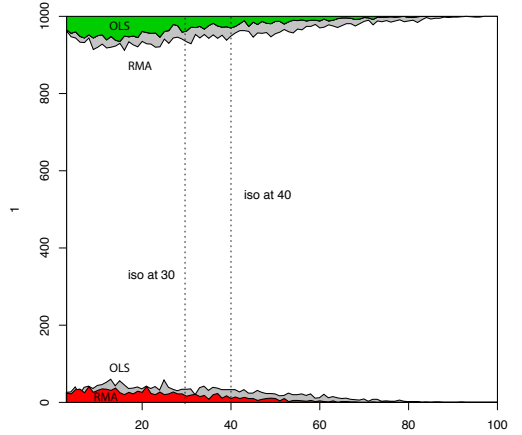
Variable 17: Slope = 0.996
