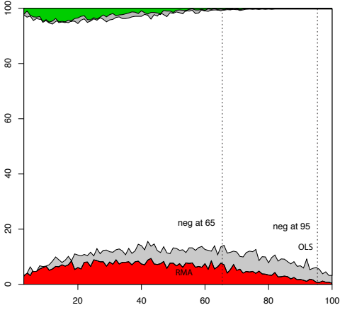
Variable 14: Slope = 0.991
