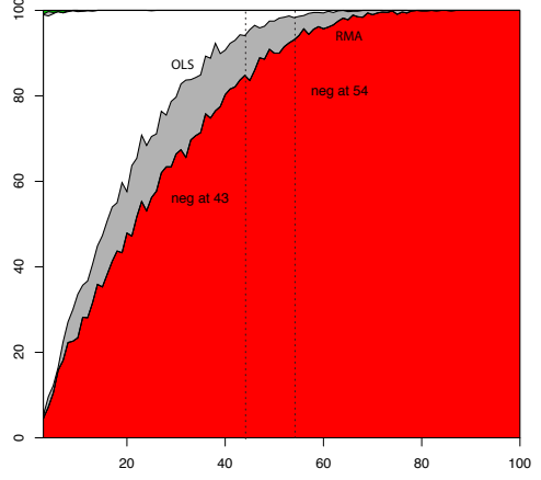
Variable 13: Slope = 0.916
