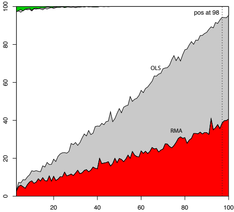
Variable 22: Slope = 0.959
