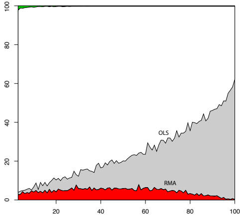
Variable 12: Slope = 0.969
