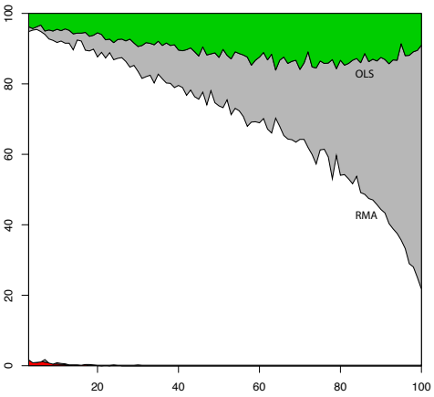
Variable 4: Slope = 1.02
