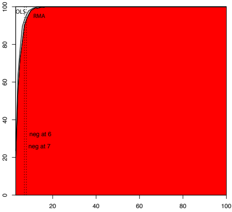
Variable 9: Slope = 0.737
