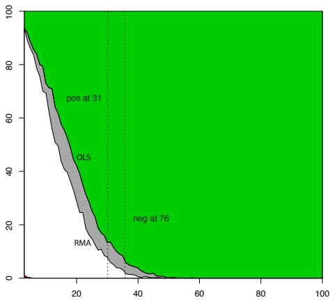
Variable 1: Slope = 1.05
