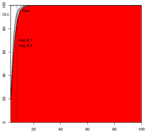
Variable 23: Slope = 0.651
