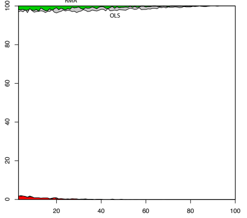
Variable 3: Slope = 1.03
