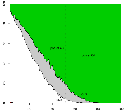
Variable 16: Slope = 1.05
