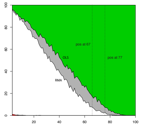
Variable 2: Slope = 1.02
