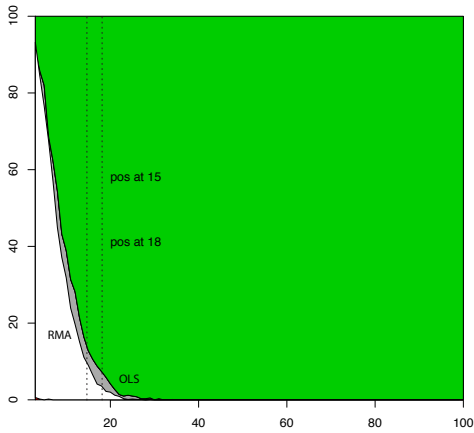
Variable 18: Slope = 1.09
