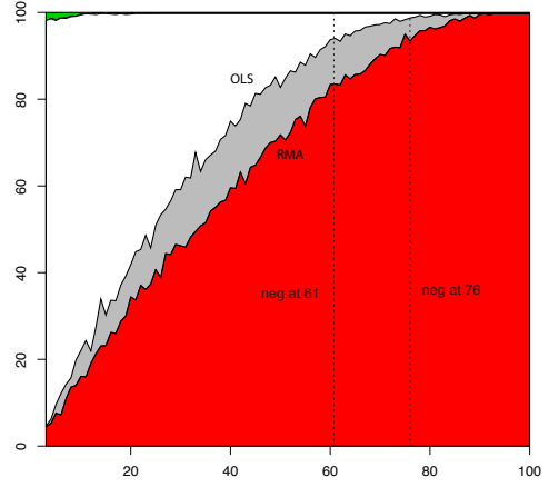
Variable 5: Slope = 0.945
