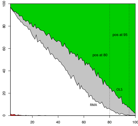
Variable 19: Slope = 1.03
