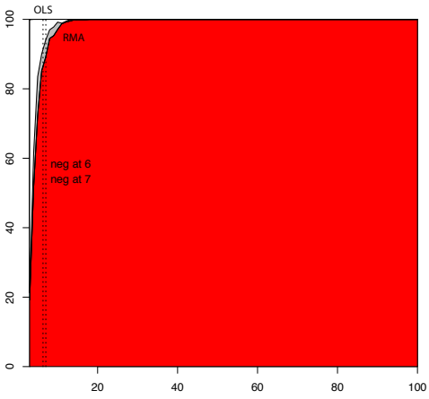
Variable 10: Slope = 0.666
