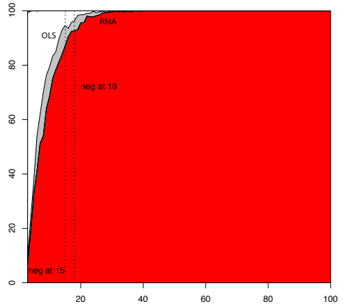
Variable 15: Slope = 0.748
