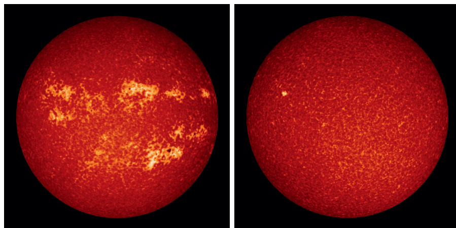
The Sun at the peak (left) and at a minimum of its activity: The Kodaikanal Observatory in India photographed our star in 1928 (left) and 1933. The images show the intensity in the calcium II line of the optical spectrum.
