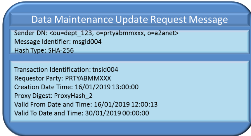
Figure 36 – Unsuccessful scenario 4 – DataMaintenanceUpdateRequestMessage
