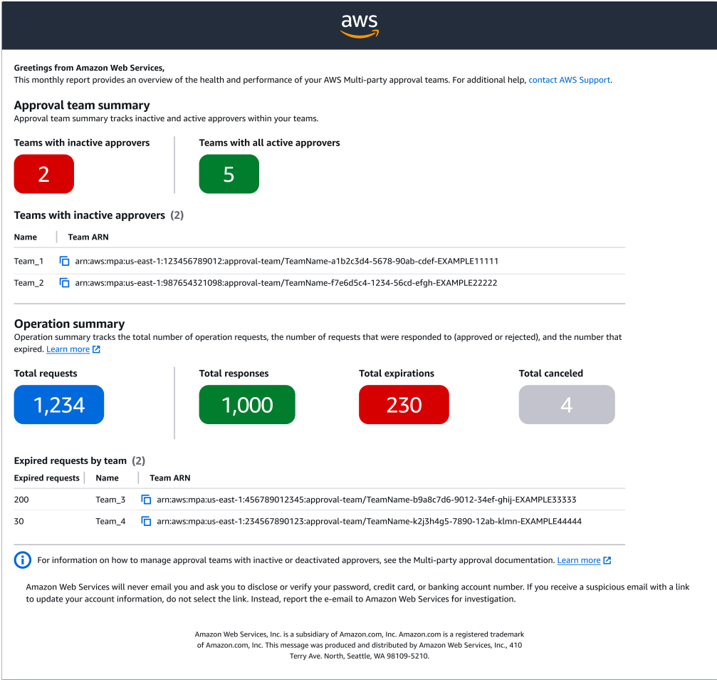
Figure 3: Diagram depicting the Multi-party approval monthly team report.
