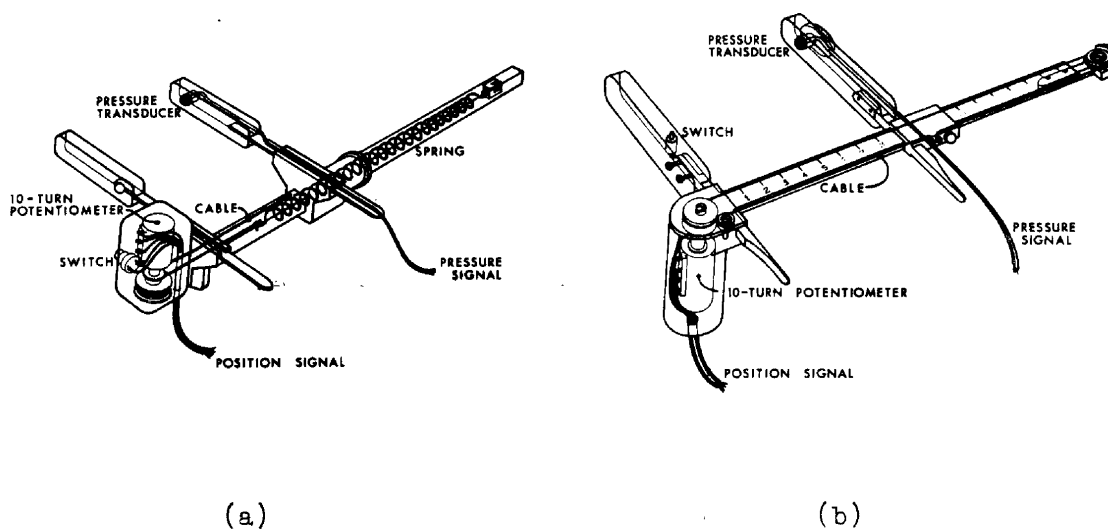
Figure 7. Drawings of modified anthropometer in (a) and modified sliding calipers in (b) showing potentiometer, pulley and cable system, and pressure transducer.
