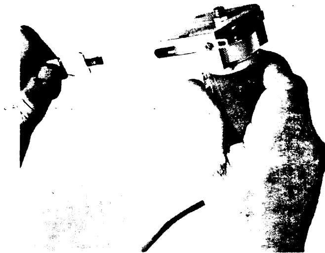
Figure 9. Modified girth device for electrical readout of circumference measurements.
