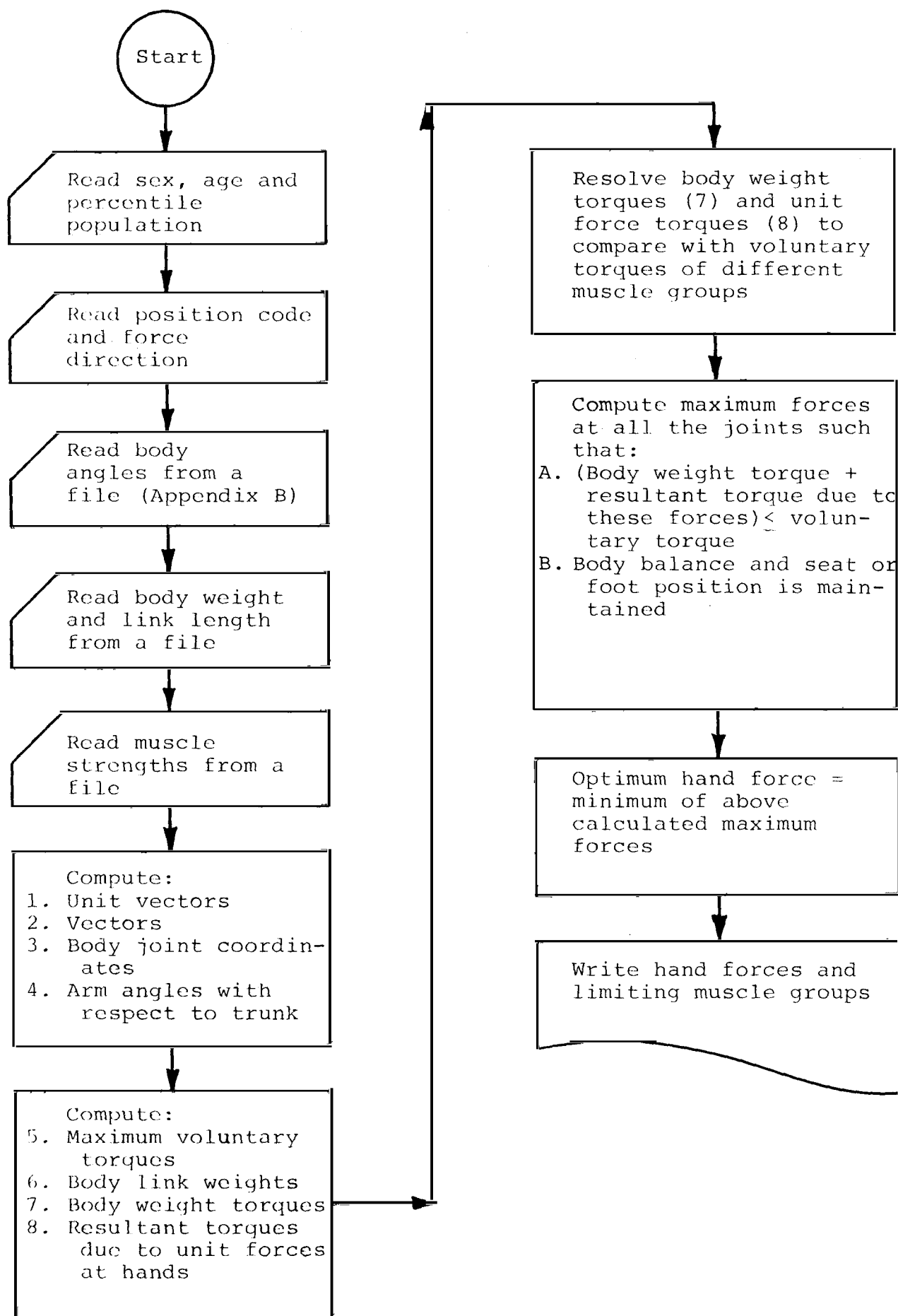
Figure 1: Macro Logic Flow Diagram
